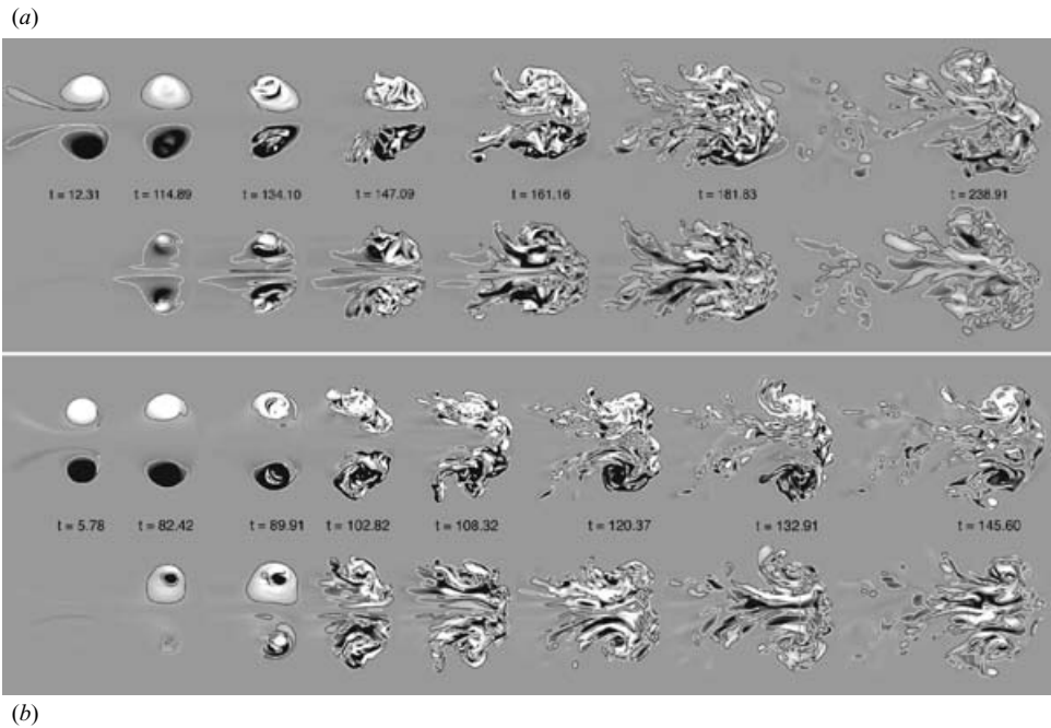
FIGURE 10. Streamwise cuts through the centre of ring A ( a ) and B ( b ). The upper part shows \omega_y , that is vorticity perpendicular to the paper plane. Contour lines denote \omega_y = \pm 0.065 (A) and \omega_y = \pm 0.146 (B), respectively. The lower part shows the streamwise vorticity \omega_z and contour lines denote \omega_z = \pm 0.065 (A), and \omega_z = \pm 0.146 (B), respectively.
